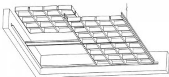
GRIDA-T (h40-15-L)
